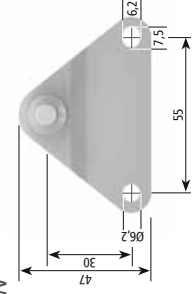
Part No. / Bestell-Nr. 8264WV F max * = 1000 N
